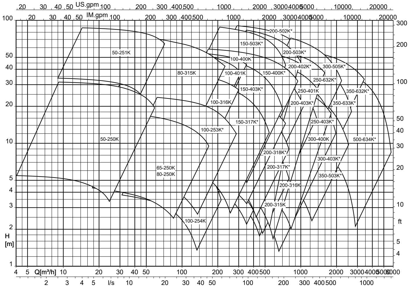
Sewatec/Sewabloc K + *K-max, n = 2900-480 rpm (speed-based selection chart)
