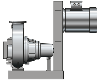
Pump set with baseplate, belt drive and belt guard
