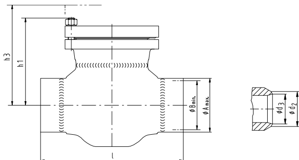
Fig. 3: Sectional drawing of STAAL 100 AKKS
