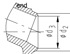
Butt weld end
