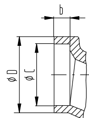
Socket weld
