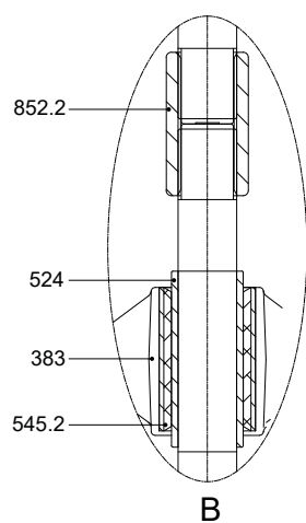
Fig. 6: Detail B
